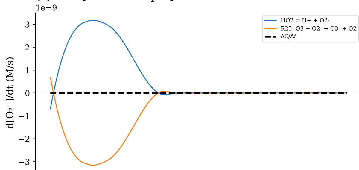
(c) O 2 - [final=0.13 pM]
