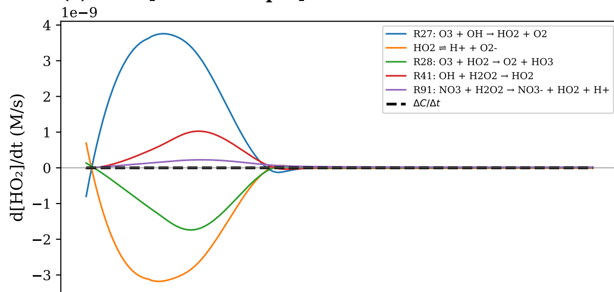
(a) HO 2 [final=0.98 pM]
