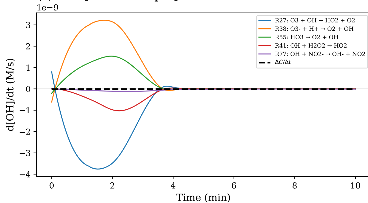
(e) OH [final=0.00 pM]
